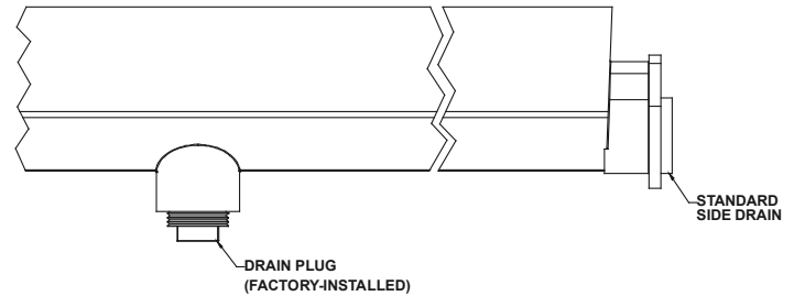
DRAIN PAN (SIDE VIEW) FIGURE 9
