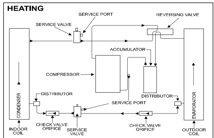
UNIT HEATING AND COOLING CYCLES FIGURE 11B
