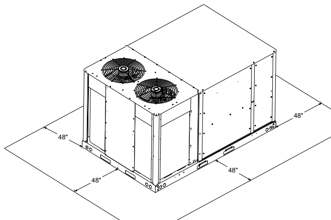
UNIT CLEARANCES
